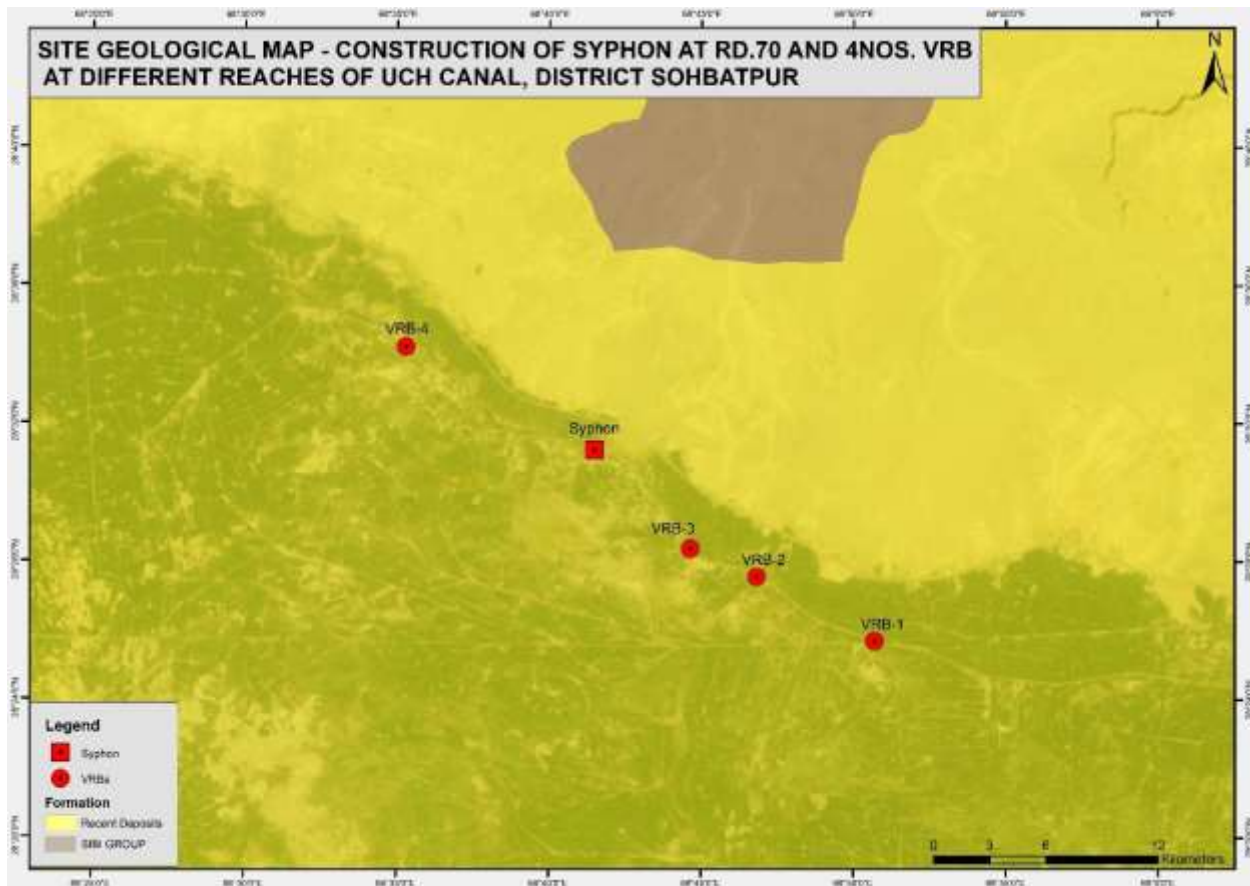
Figure-3-4: Surface geological map of the Construction Site.
